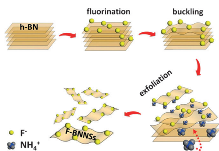
Figure 3. Illustration of the fluorination-assisted exfoliation mechanism. The exfoliating process involves the following sequence: fluorination, buckling of the sheets on the surface, insertion of ammonium ions, and exfoliation of sheets.
